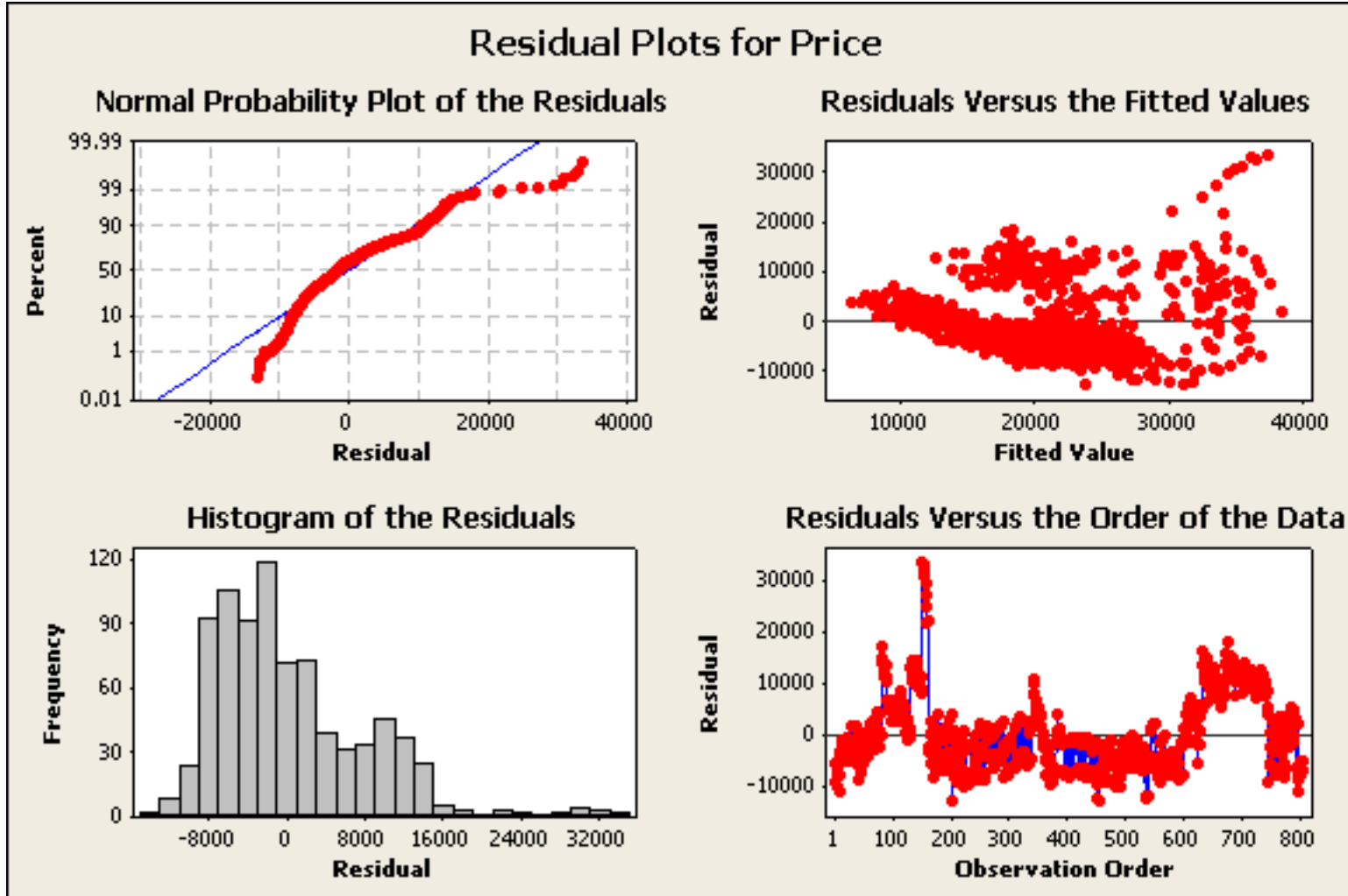
Figure 3: Residual plots for Equation 2.
