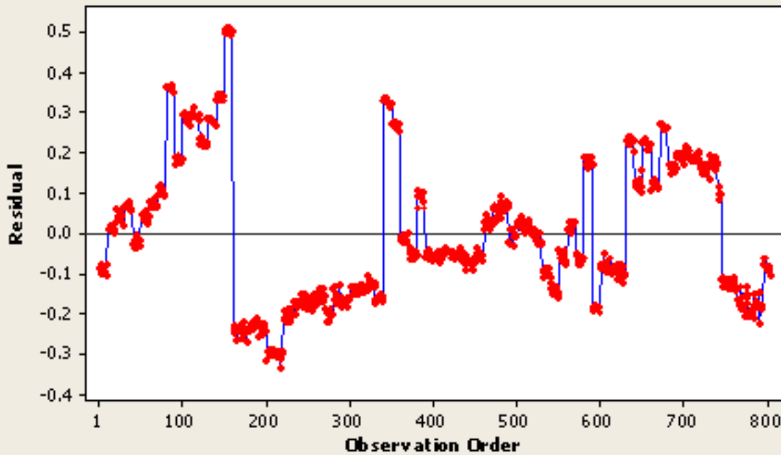
Figure 4: A residual versus order plot using Equation 1: \text{Price} = 24723 - 0.17 \text{ Mileage} .
