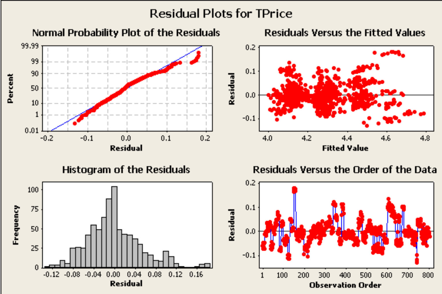
Figure 5: Minitab plots of the residuals for the Equation 3: TPrice = 3.98 - 0.000003 Mileage +
